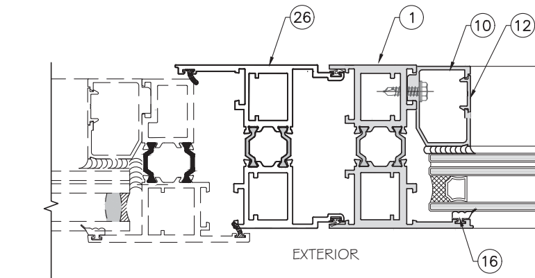
CASEMENT – FIXED MULLION MULLION DETAIL
