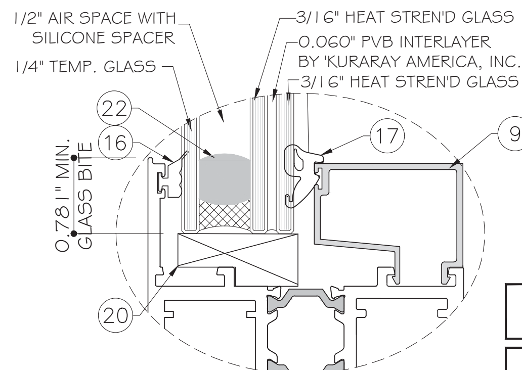
GLASS TYPE 'G1-2' 1 3/16" NOMINAL OVERALL
