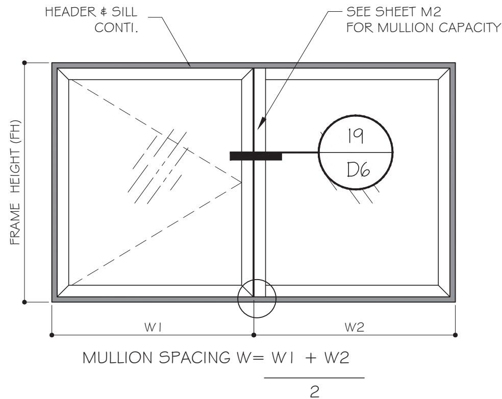
FIXED WINDOW WITH CASEMENT OPTION NOTE: CASEMENT OR PROJECTED OUT WINDOW UNDER A SEPARATE APPROVAL
