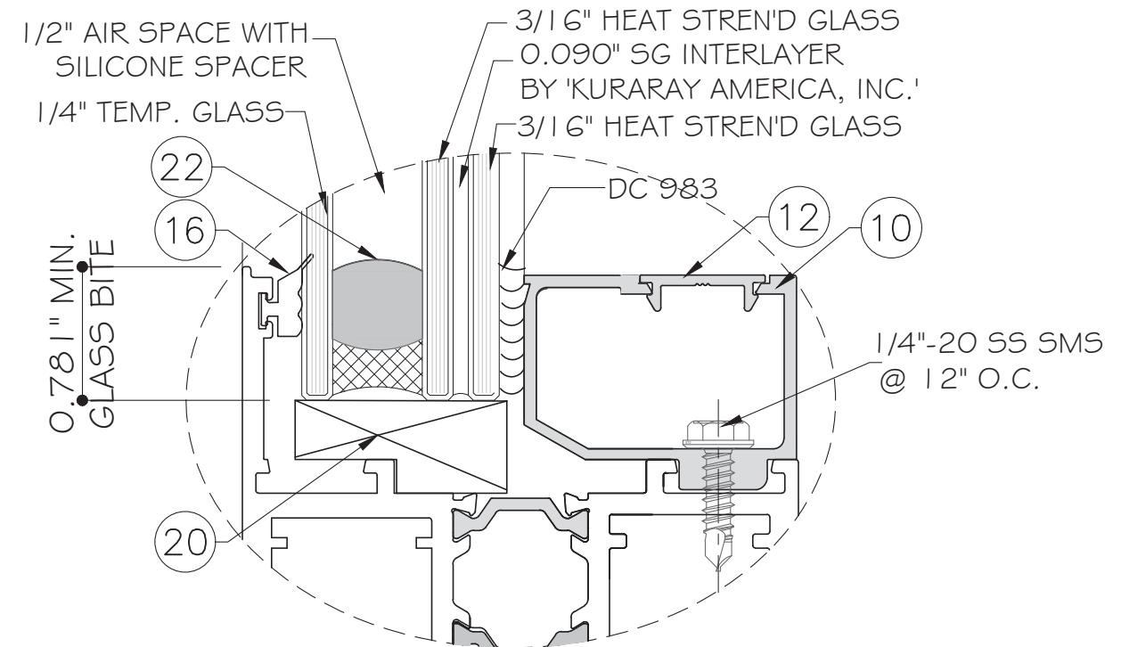
GLASS TYPE 'G1-2' 1 3/16" NOMINAL OVERALL
