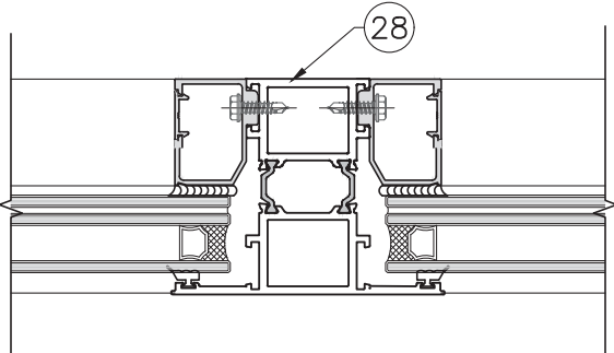
FIXED – FIXED MULLION MULLION DETAIL
