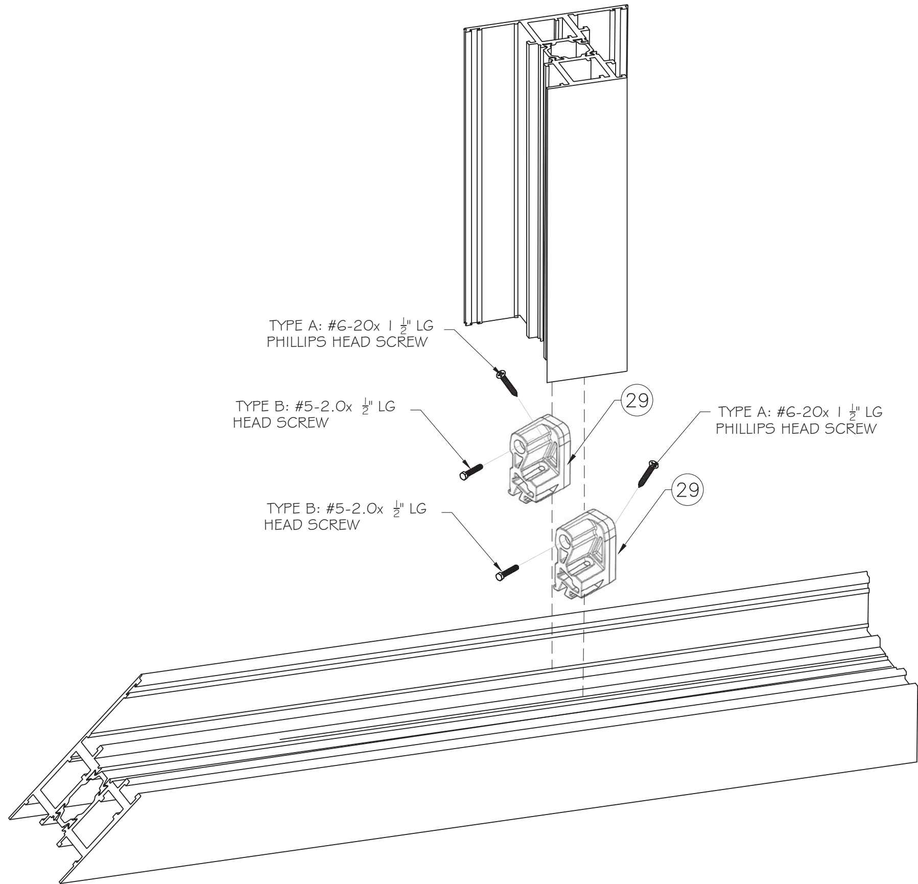
"T" - JUNCTION CONNECTION
