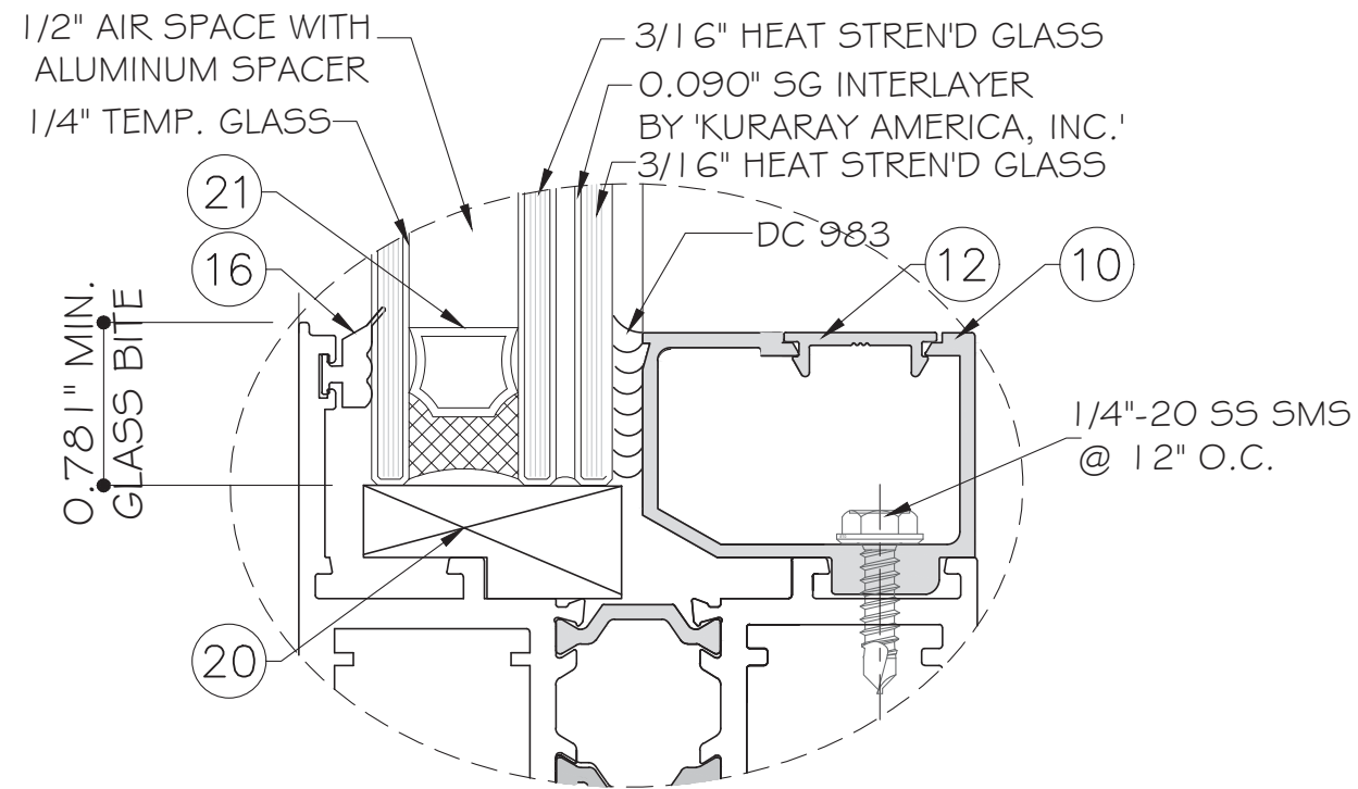
GLASS TYPE 'G1-1' 1 3/16" NOMINAL OVERALL LARGE MISSILE IMPACT
