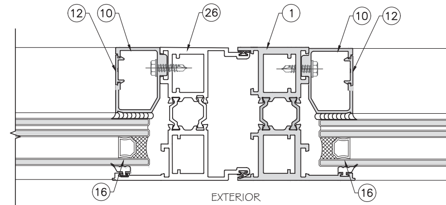
FIXED — FIXED MULLION MULLION DETAIL
