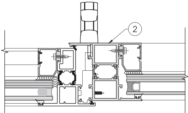
CASEMENT – FIXED MULLION MULLION DETAIL
