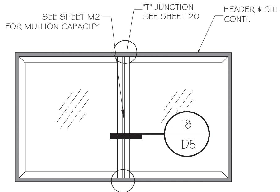
FIXED - FIXED OPTION
